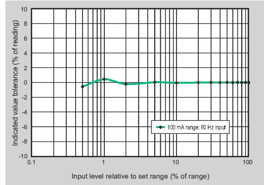
Example of WT210 Current Accuracy
