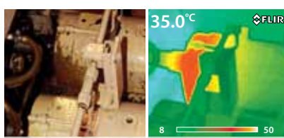
Motor: Lagerproblem.
